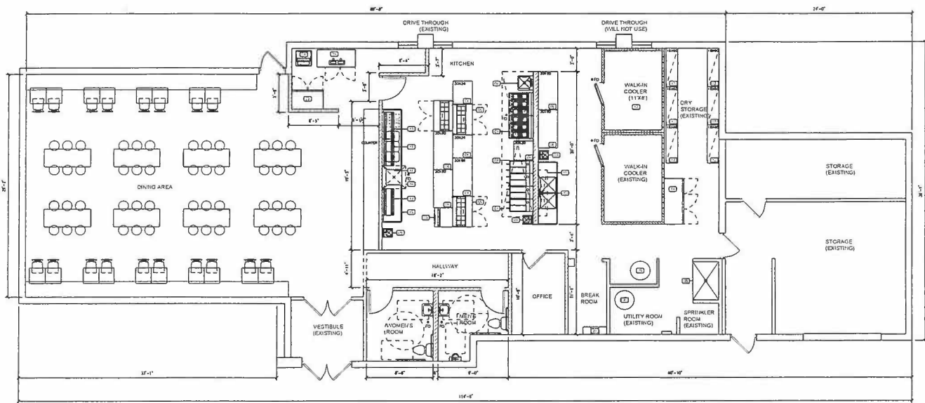
1 FLOOR PLAN 1/4"=1'-0"
